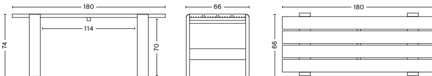
WEEKDAY TABLE 180 LENGTH 180 CM | 70.75" WIDTH 66 CM | 26" HEIGHT 74 CM | 29.25"
