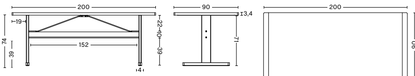
PASSERELLE TABLE | VENEER TABLETOP WIDTH 200 CM | 78.75" DEPTH 90 CM | 35.5" HEIGHT 74 CM | 29.25" CROSSBAR HEIGHT 39 CM | 15.5"
