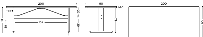
PASSERELLE TABLE | LINOLEUM | LAMINATE TABLETOP WIDTH 200 CM | 78.75" DEPTH 90 CM | 35.5" HEIGHT 74 CM | 29.25" CROSSBAR HEIGHT 39 CM | 15.5"
