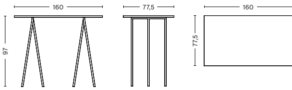
LOOP STAND HIGH L160 LENGTH 160 CM | 62.99" WIDTH 77,5 CM | 30.51" HEIGHT 97 CM | 38.19"
