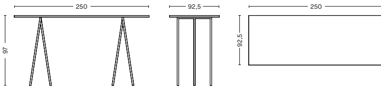
LOOP STAND HIGH L250 LENGTH 250 CM | 98.43" WIDTH 92,5 CM | 36.42" HEIGHT 97 CM | 38.19"
