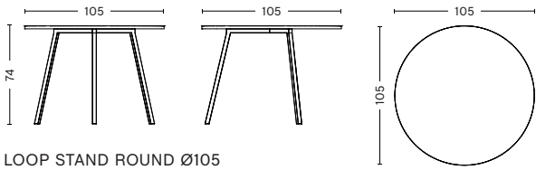
LOOP STAND ROUND Ø105 DIAMETER 105 CM | 41.34" HEIGHT 74 CM | 29.13"
