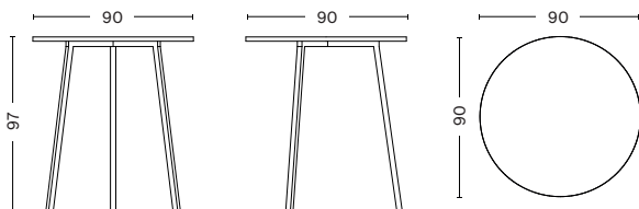
LOOP STAND ROUND Ø90 DIAMETER 90 CM | 35.43" HEIGHT 97 CM | 38.19"
