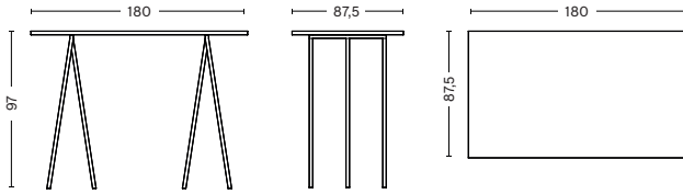
LOOP STAND HIGH L180 LENGTH 180 CM | 70.87" WIDTH 87,5 CM | 34.45" HEIGHT 97 CM | 38.19"
