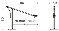
FIFTY-FIFTY TABLE LAMP WITH TABLE BASE WIDTH 18,5 CM | 7.3" DEPTH 90 CM | 35.4" HEIGHT 60 CM | 23.6" MAX. ARM REACH 75 CM | 29.5"
