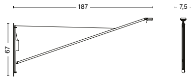
FIFTY-FIFTY WALL LAMP WIDTH 7.5 CM | 3" DEPTH 187 CM | 73.6" HEIGHT 67 CM | 26.4"
